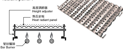
爐頭連熱反射板示意 Diagram of burner with heat radiant panel.
